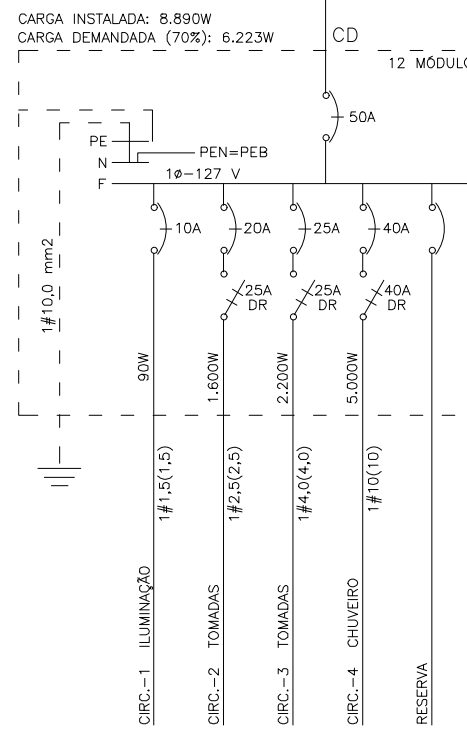
DIAGRAMA UNIFILAR
