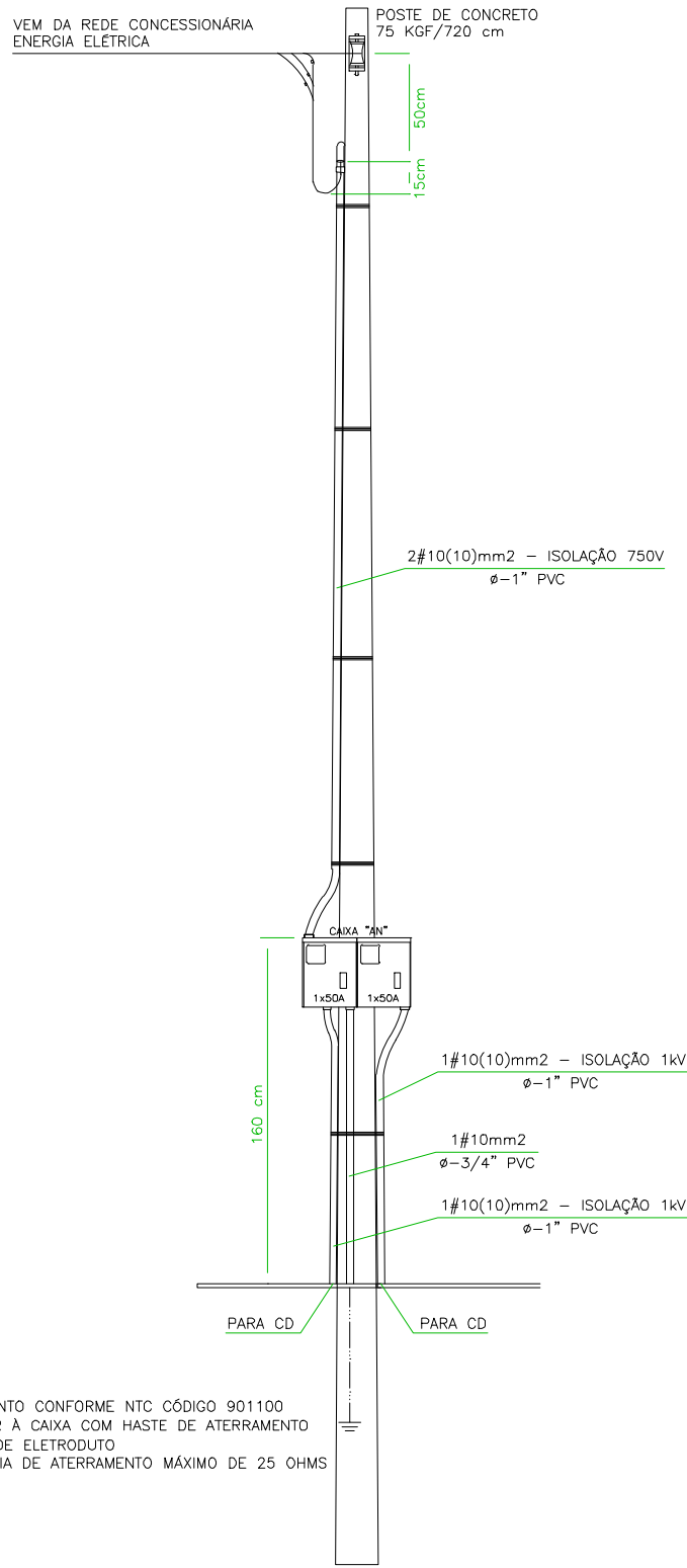
VISTA FRONTAL
